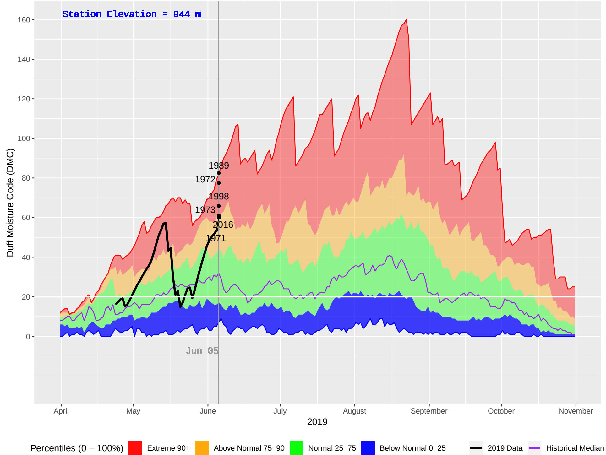
GRASSY PLAINS HUB (161) : Historical (1970–2018), Current (2019) Daily Duff Moisture Code (DMC)
