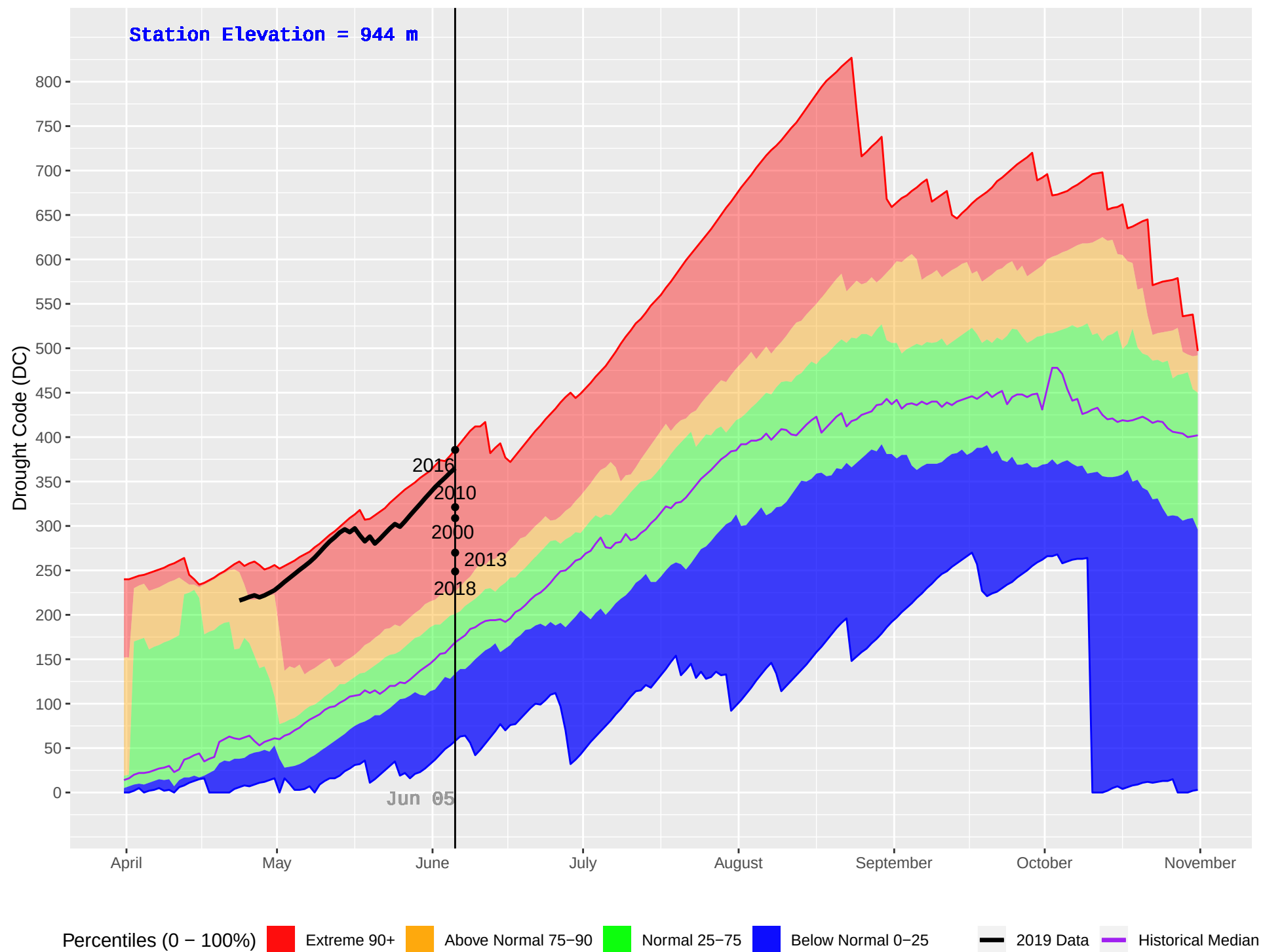
GRASSY PLAINS HUB (161) : Historical (1970–2018) and Current (2019) Daily Drought Code (DC)
