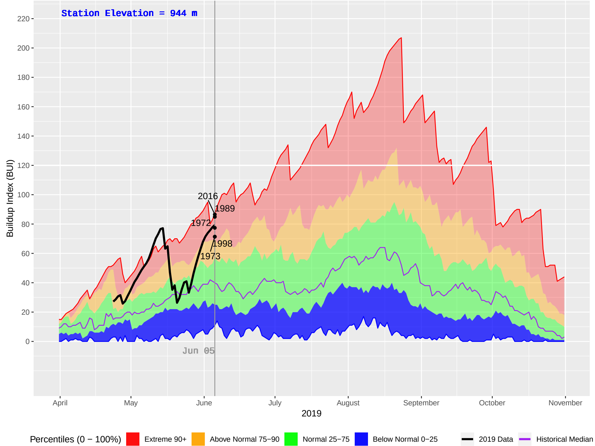
GRASSY PLAINS HUB (161) : Historical (1970–2018), Current (2019) Daily Buildup Index (BUI)
