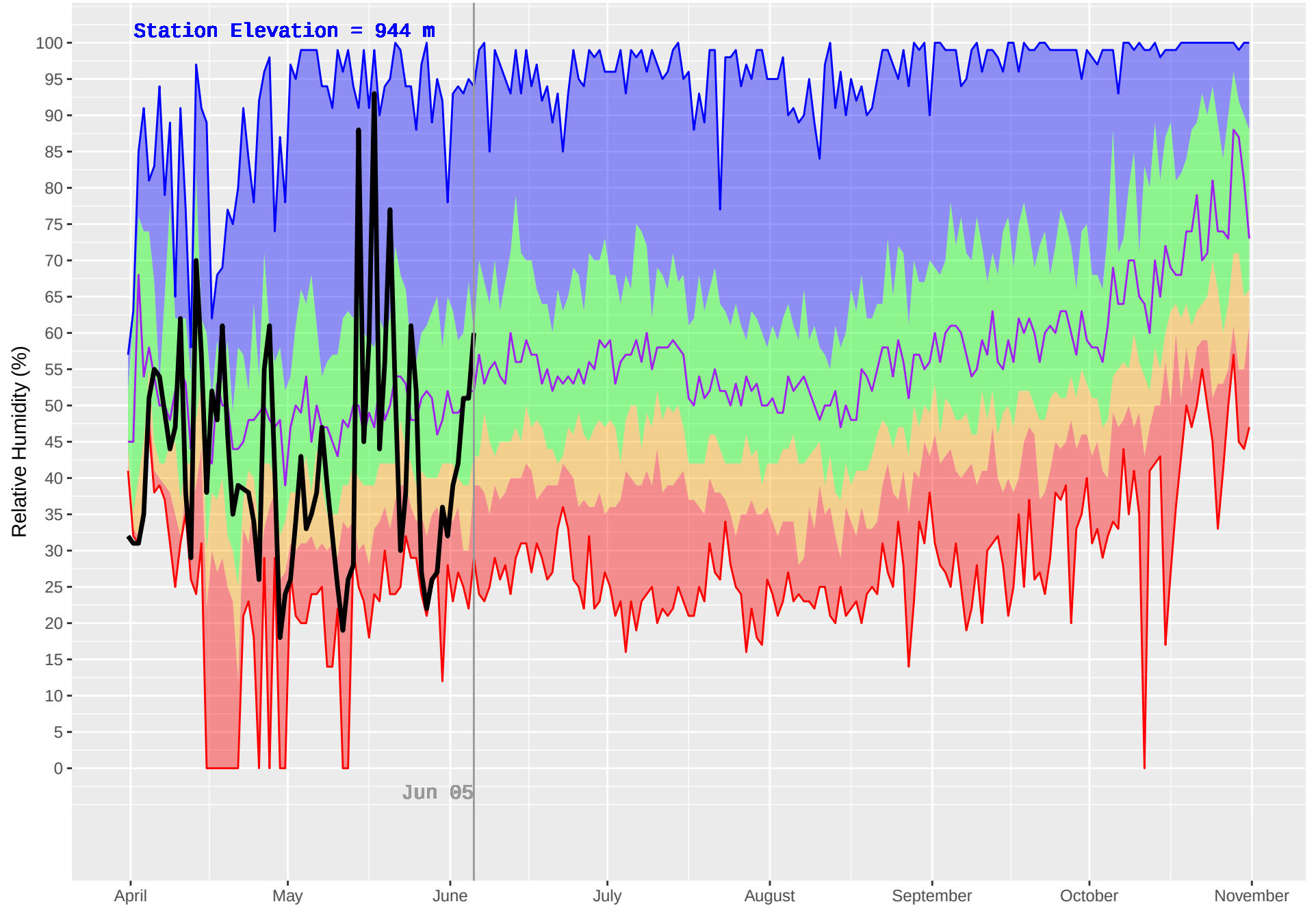
GRASSY PLAINS HUB (161) : Historical (1970–2018) and Current (2019) Daily Relative Humidity
