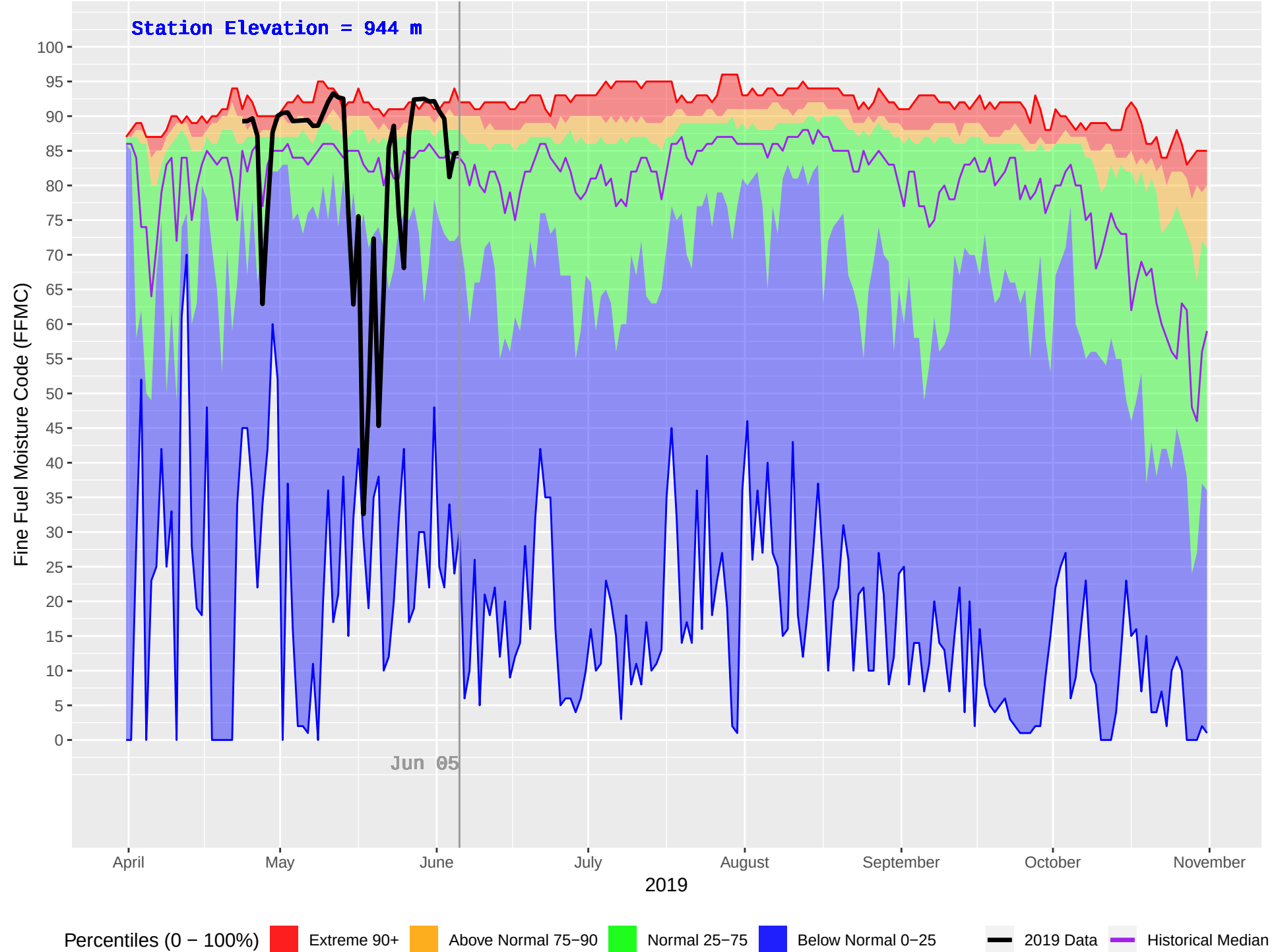
GRASSY PLAINS HUB (161) : Historical (1970–2018) and Current (2019) Daily Fine Fuel Moisture Code (FFMC)
