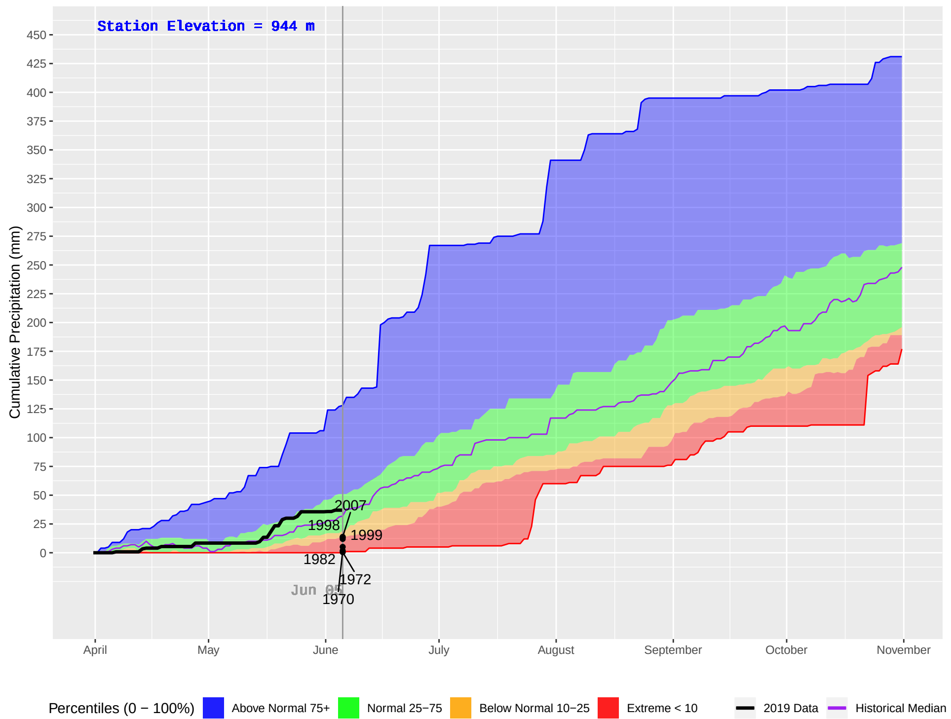
GRASSY PLAINS HUB (161) : Historical (1970–2018), Current (2019) Daily Cumulative Precipitation
